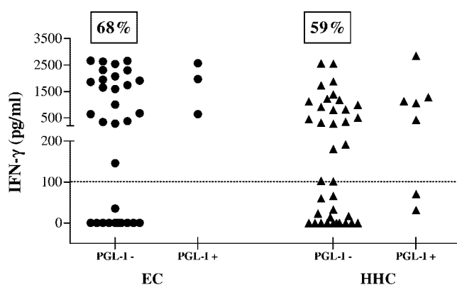
FIG. 3. Added value of in vitro T-cell responses to M. leprae antigens. The highest level of IFN- \gamma production induced by PBMC against ML1989, ML1990, ML2283, ML2346, or ML2567 is depicted for EC individuals (●) and HHCs (▲) in the context of their seropositivity for antibodies against PGL-I. The percentages of individuals lacking antibodies against PGL-I (PGL-I-) and those responding to \geq 1 of the M. leprae -unique proteins are indicated above the figure. The total numbers of individuals that recognize a certain peptide are indicated in boxes. The threshold for positive responses is indicated by the dotted line.
