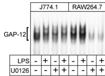
FIG. 6. Effect of U0126 on the DNA-binding activity of GAP-12. Nuclear extracts of the cells pretreated with U0126 and stimulated with LPS (as described in the legend for Fig. 5) for 1 h were prepared and subjected to EMSA to evaluate the DNA-binding activities of GAP-12. Similar results were obtained in three independent experiments.
